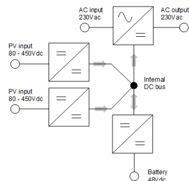
Inside the Multi RS Solar dual tracker
